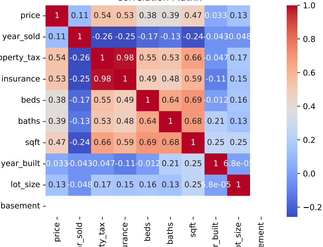
Correlation Matrix
